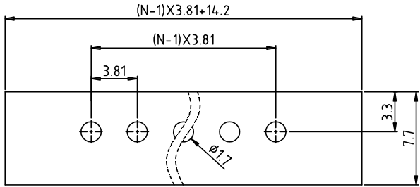
PCB. LAYOUT I
