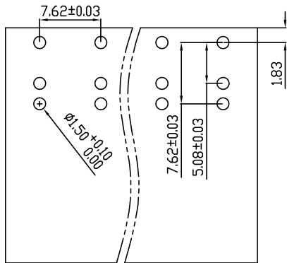
PCB LAYOUT
