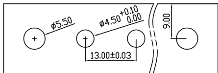
PCB Layout
