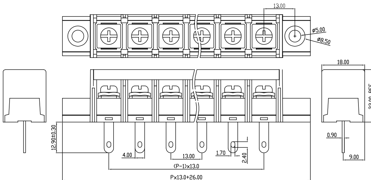
PCB Layout
