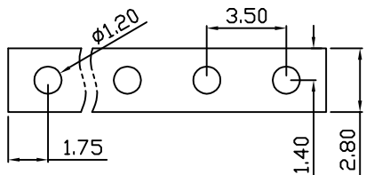
PCB Layout
