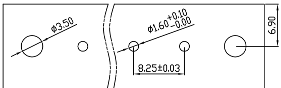
PCB Layout
