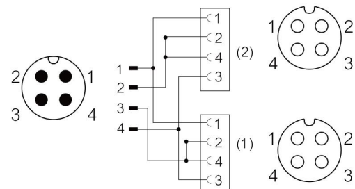
Contact assignment of M12 Y2/T2 connector
